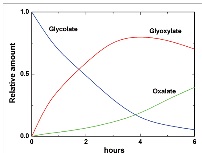
FIGURE 7 | Oxidation of glycolate and glyoxylate and formation of glyoxylate and oxalate by glycolate oxidase from wheat leaves. The changes of concentrations of glycolate, glyoxylate, and oxalate are calculated according to the kinetic equations based on the values of kinetic constants given in Table 1. Incorporation of the label from 1\text{-}^{14}\text{C} -glycolate to glyoxylate and oxalate in the reaction catalyzed by the purified glycolate oxidase revealed a similar profile (Igamberdiev et al., 1988).
