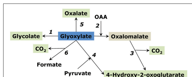
FIGURE 8 | Pathways of glyoxylate conversion in plants. (1) reduction to glycolate; (2) non-enzymatic condensation with oxaloacetate (OAA) forming oxalomalate; (3) the latter is decarboxylated to 4-hydroxy-2-oxoglutarate; (4) enzymatic condensation with pyruvate forming 4-hydroxy-2-oxoglutarate; (5) oxidation to oxalate; (6) decarboxylation to formate.
